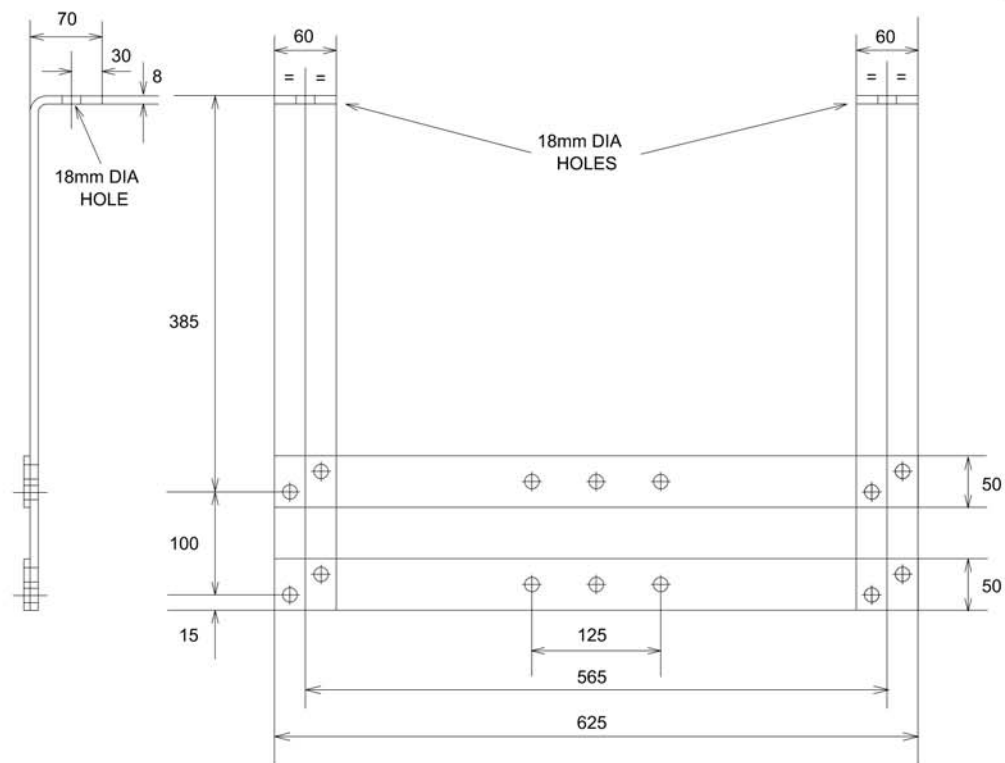
ITEM 14 60 x 8 AND 50 x 6 FLAT BAR TO UTILISE WOOD BLOCK TO 0309/1
